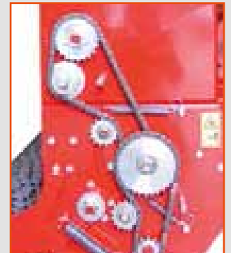
Seed distribution engaged by ASA 50 chain transmission
